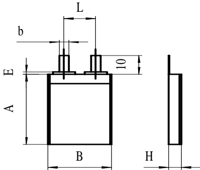
Cell or adding Ni tabs
