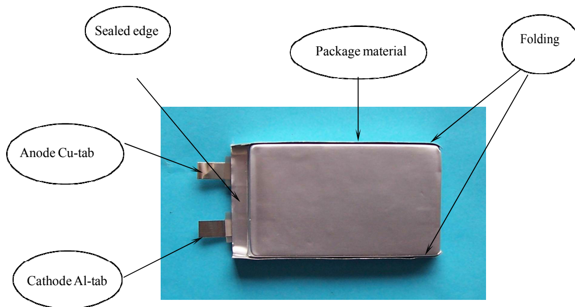
Exterior schematic of polymer lithium-ion cells
