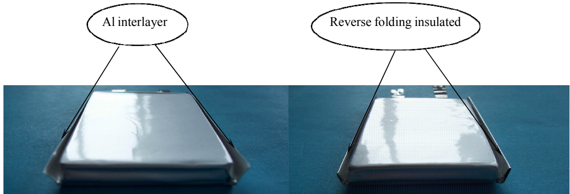
Single folding edge schematic of PL cells
